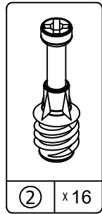
② x16 #A22610 cam bolt perno de leva boulon de came
